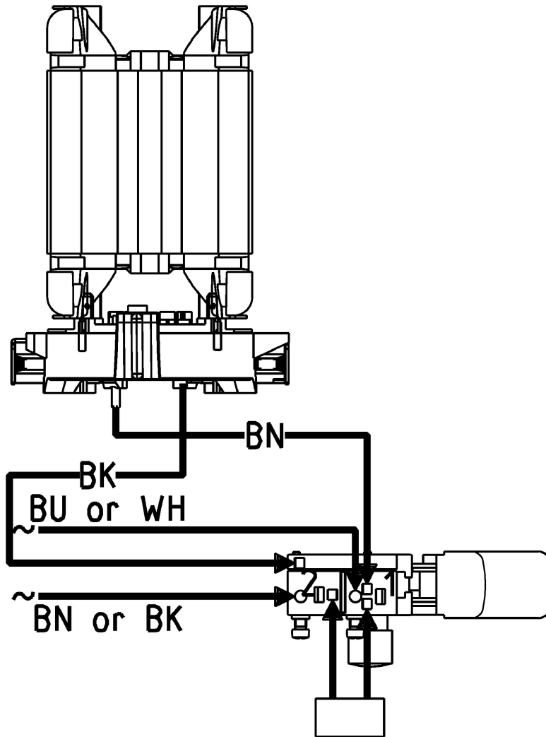
Circuit Block Diagram
