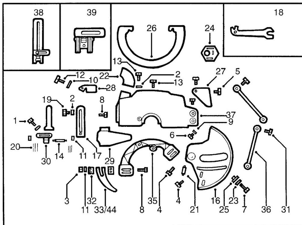
GUARD ASSEMBLY
