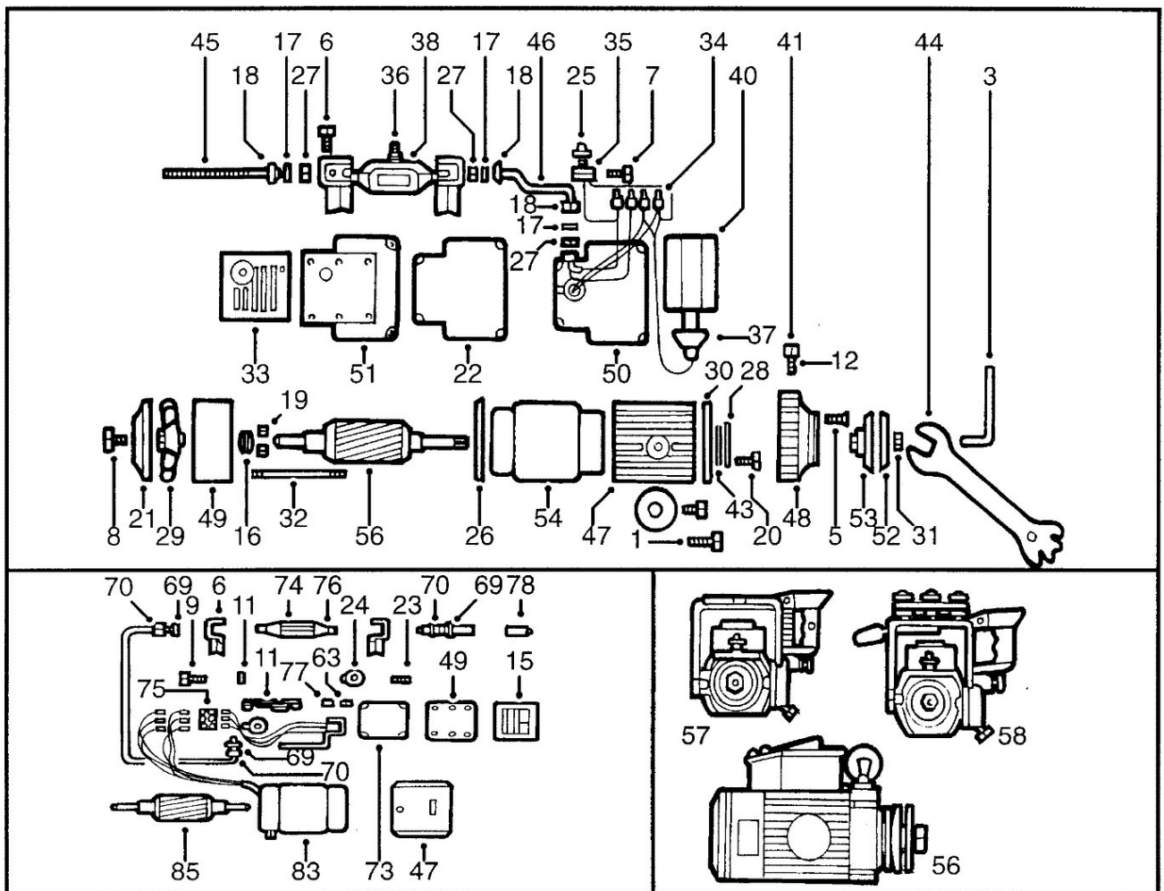
MOTOR ASSEMBLY
