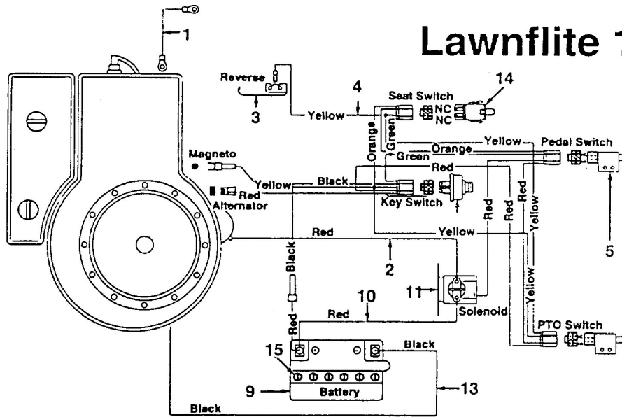
PARTS LIST FOR ELECTRICAL SYSTEM
