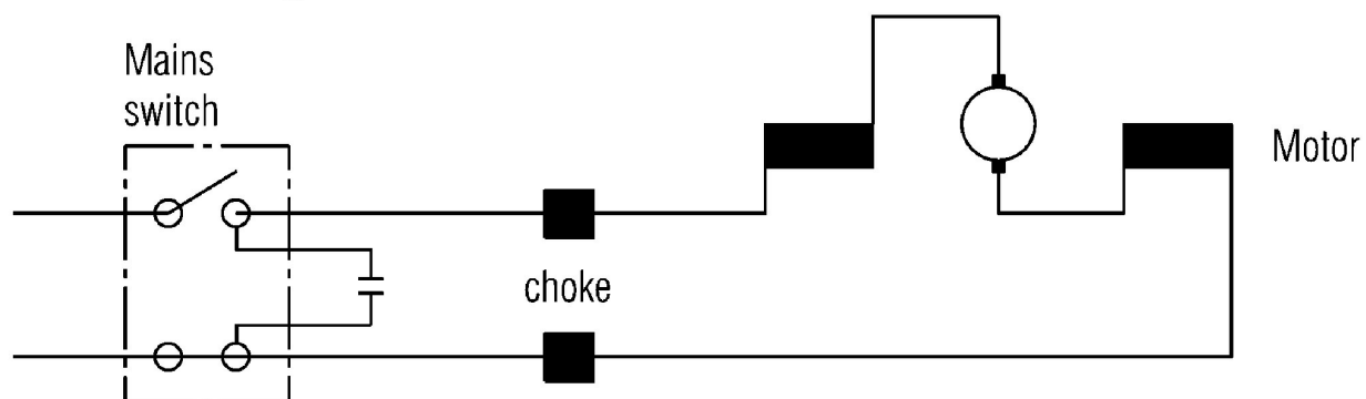
Circuit Block Diagram
