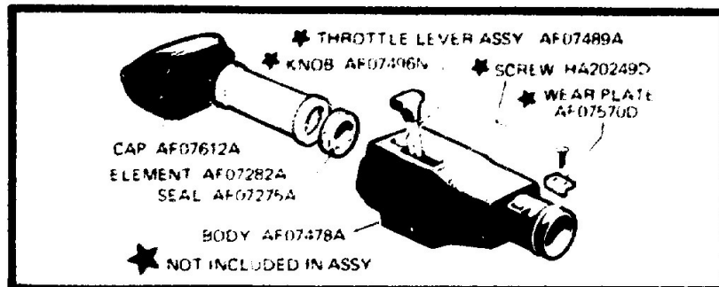
AIR FILTER ASSY. AF07480A
