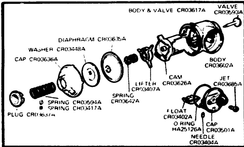
CARBURETTOR ASSY. CR03678A
