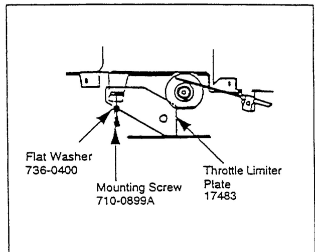
Twin Cylinder Vanguard
